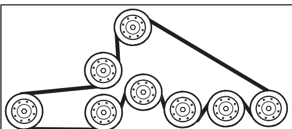
42" HIGH GRASS MULCHER DECK DRIVE BELT PATH
